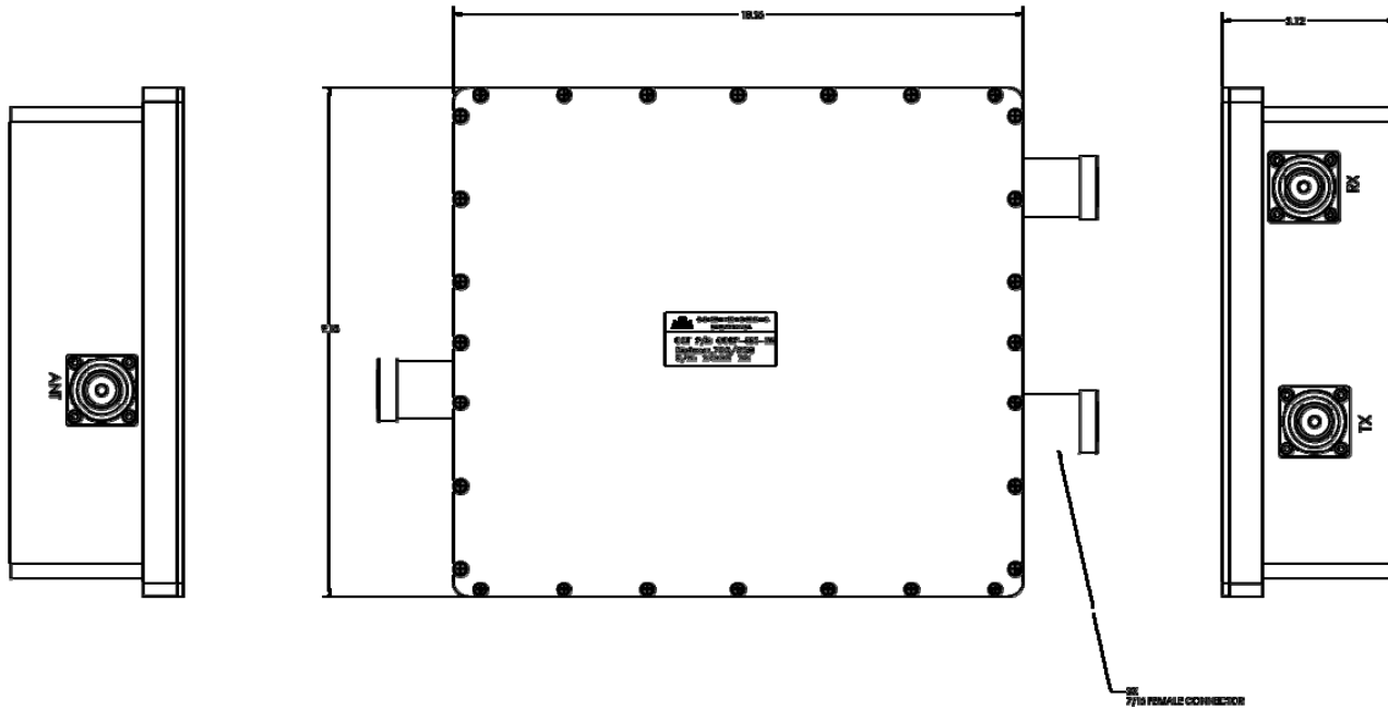
OUTLINE DRAWING
