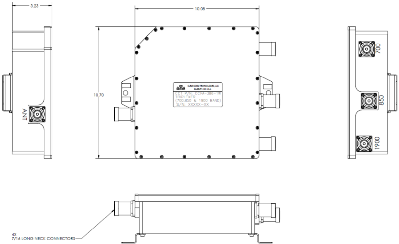
OUTLINE DRAWING
