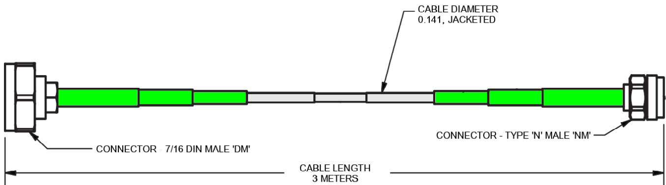
Typical Low PIM Cable Assembly
