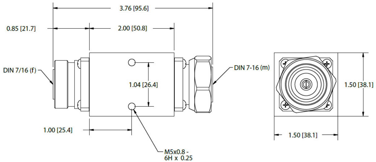
DC BLOCK - OUTLINE
